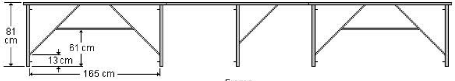
Frame Front View
